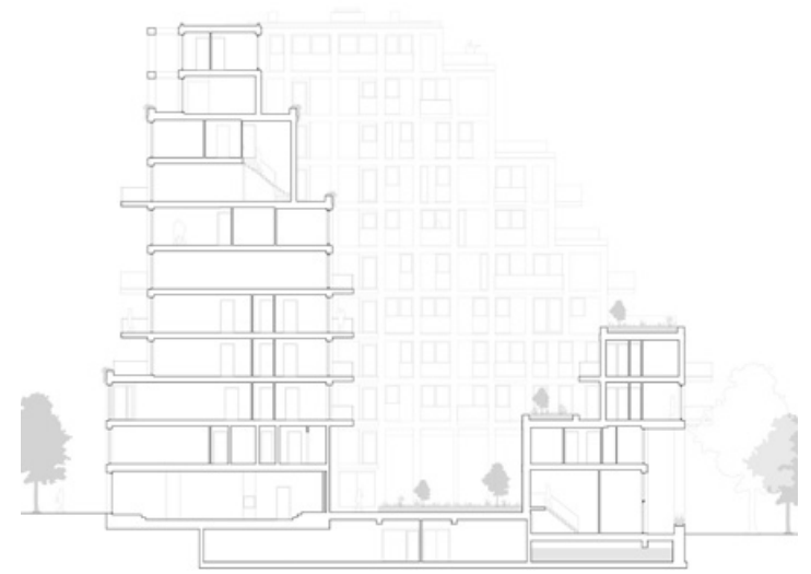
Doorsnede MO*town Track 8
